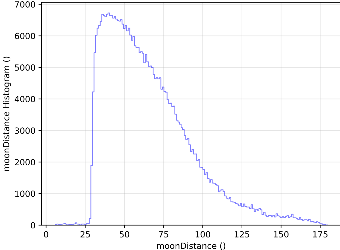
too_elab_heavy_r128_d2_griz_v3.4_10yrs WFD y band: moonDistance Histogram
