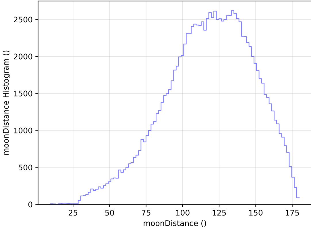
too_elab_heavy_r128_d2_griz_v3.4_10yrs WFD u band: moonDistance Histogram
