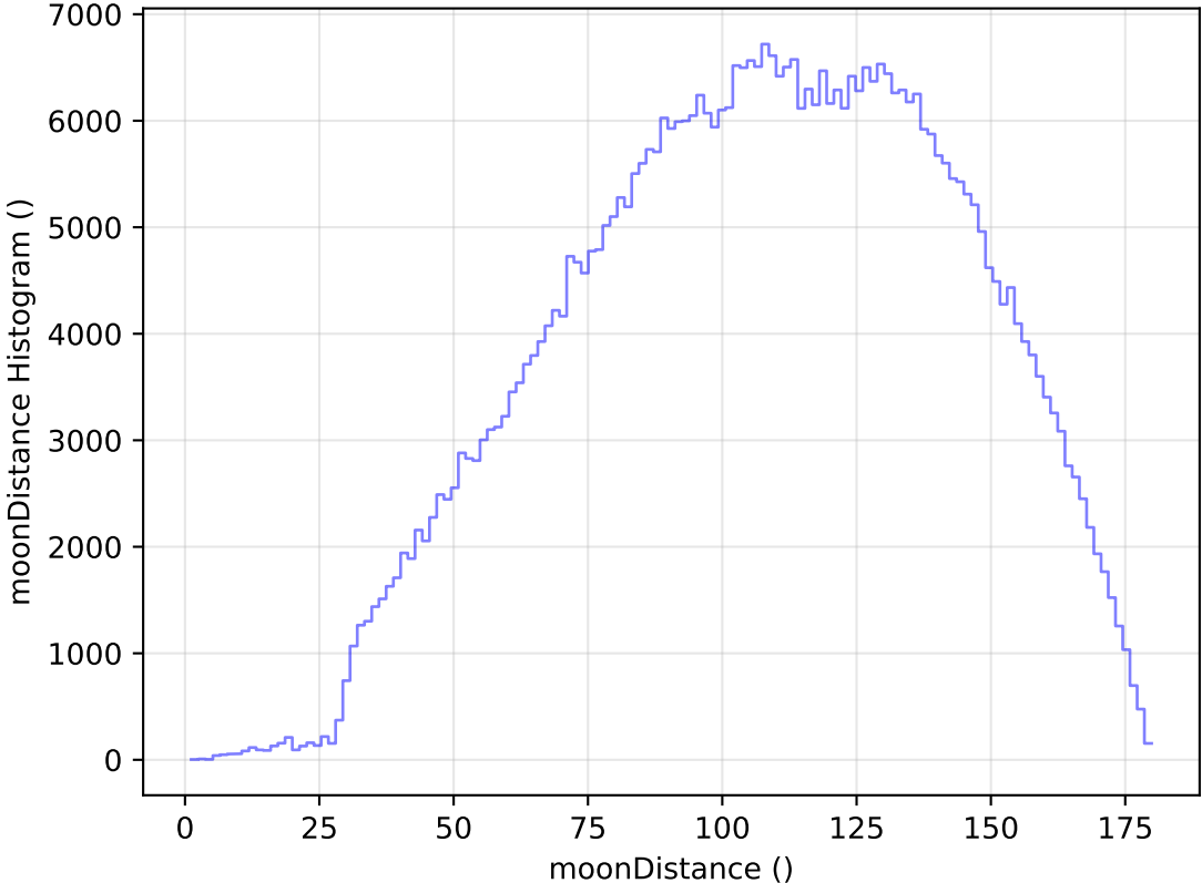
too_elab_heavy_r128_d2_griz_v3.4_10yrs WFD r band: moonDistance Histogram
