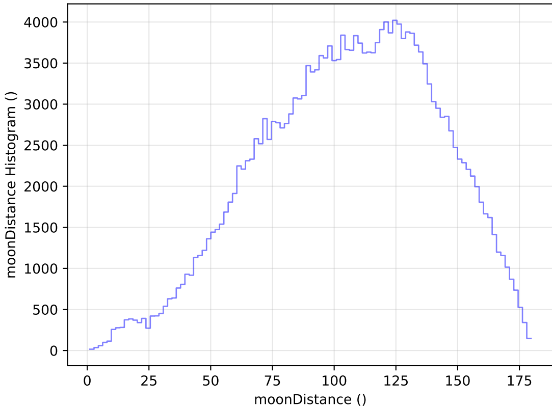
too_elab_heavy_r128_d2_griz_v3.4_10yrs WFD g band: moonDistance Histogram
