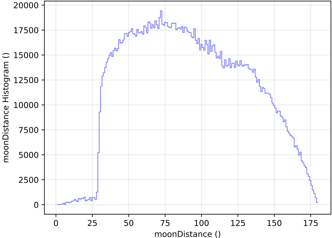
too_elab_heavy_r128_d2_griz_v3.4_10yrs WFD all bands: moonDistance Histogram
