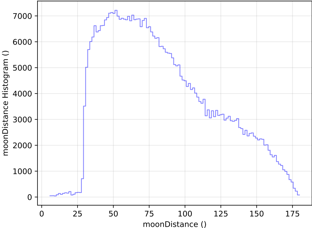
too_elab_heavy_r128_d2_griz_v3.4_10yrs All sky z band: moonDistance Histogram
