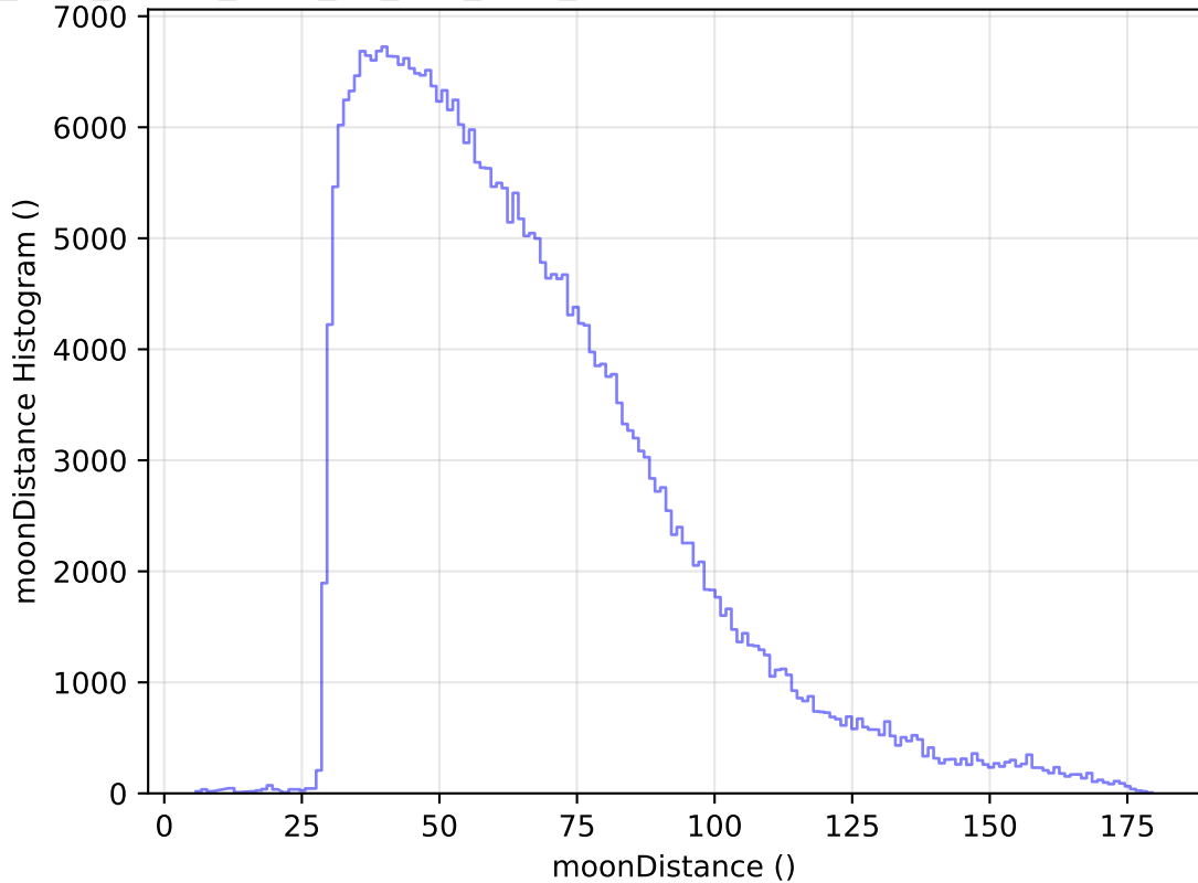
too_elab_heavy_r128_d2_griz_v3.4_10yrs All sky y band: moonDistance Histogram
