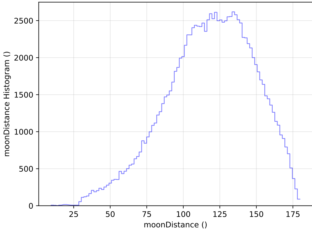
too_elab_heavy_r128_d2_griz_v3.4_10yrs All sky u band: moonDistance Histogram
