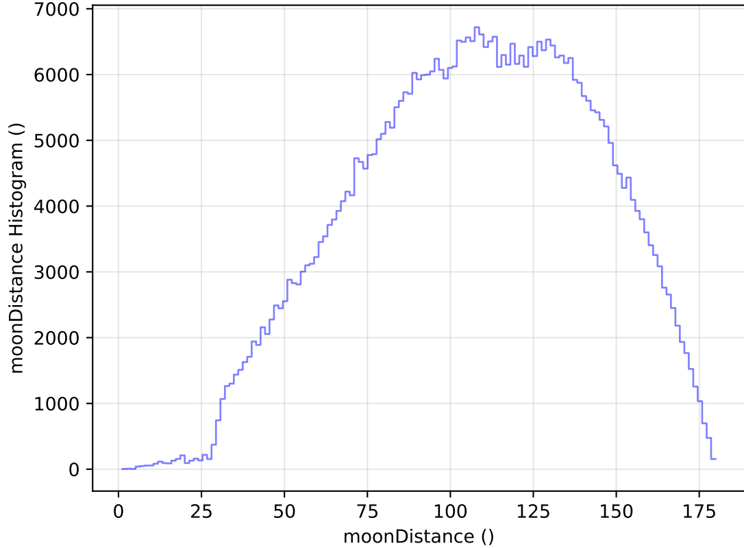
too_elab_heavy_r128_d2_griz_v3.4_10yrs All sky r band: moonDistance Histogram
