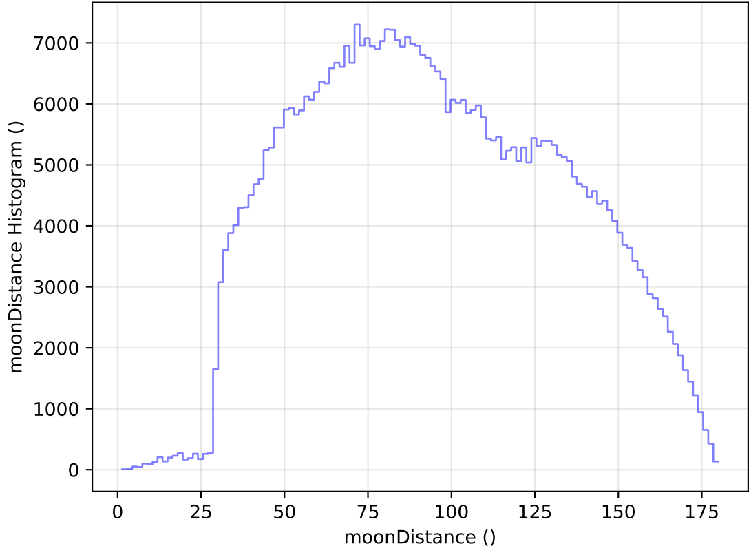
too_elab_heavy_r128_d2_griz_v3.4_10yrs All sky i band: moonDistance Histogram
