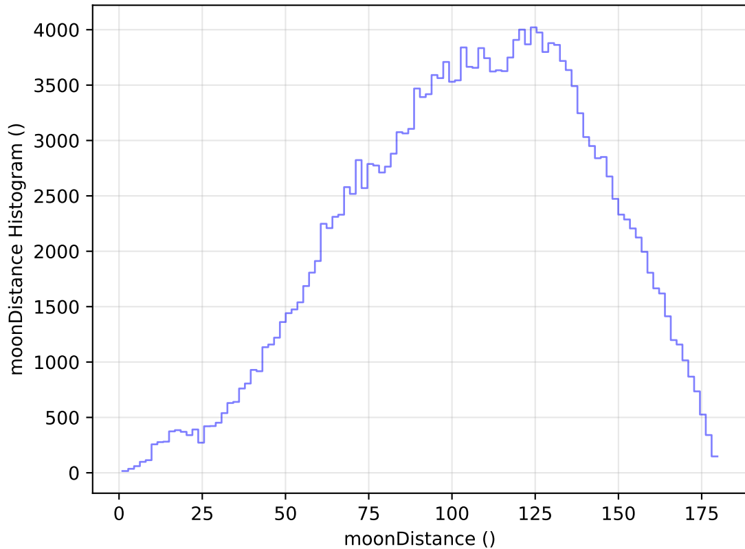
too_elab_heavy_r128_d2_griz_v3.4_10yrs All sky g band: moonDistance Histogram
