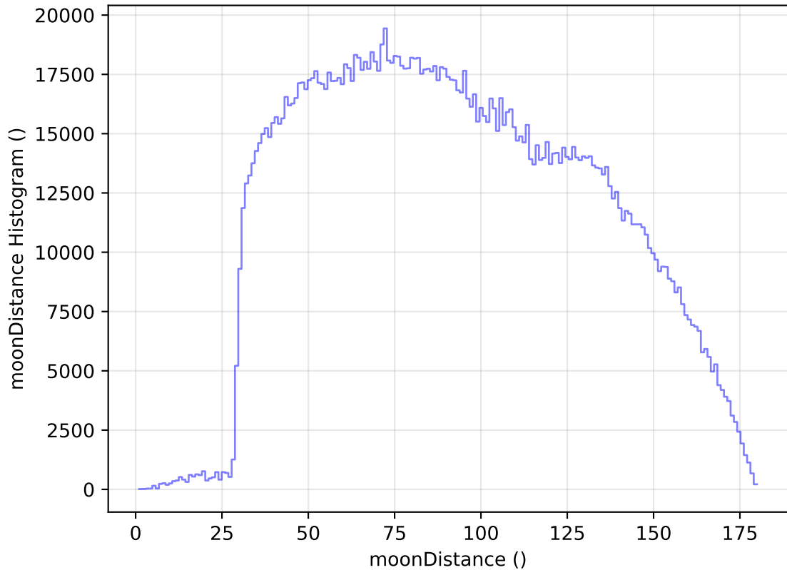
too_elab_heavy_r128_d2_griz_v3.4_10yrs All sky all bands: moonDistance Histogram
