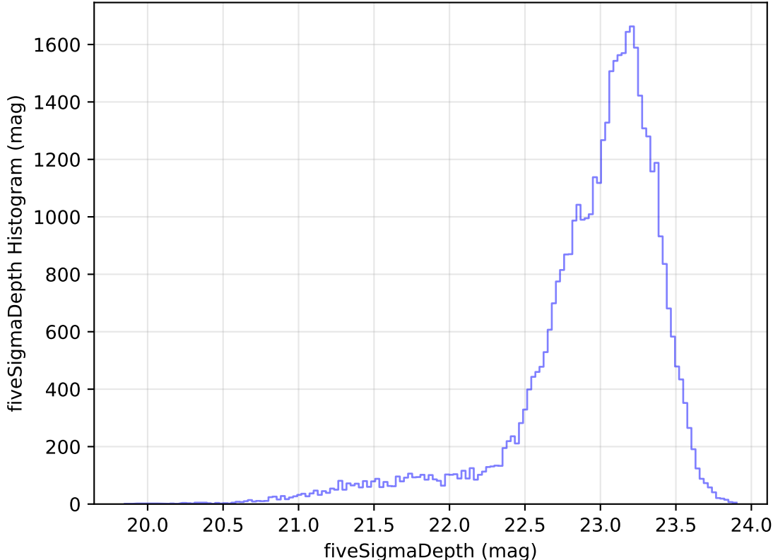
too_elab_heavy_r128_d2_griz_v3.4_10yrs Yr 1 z band: fiveSigmaDepth Histogram
