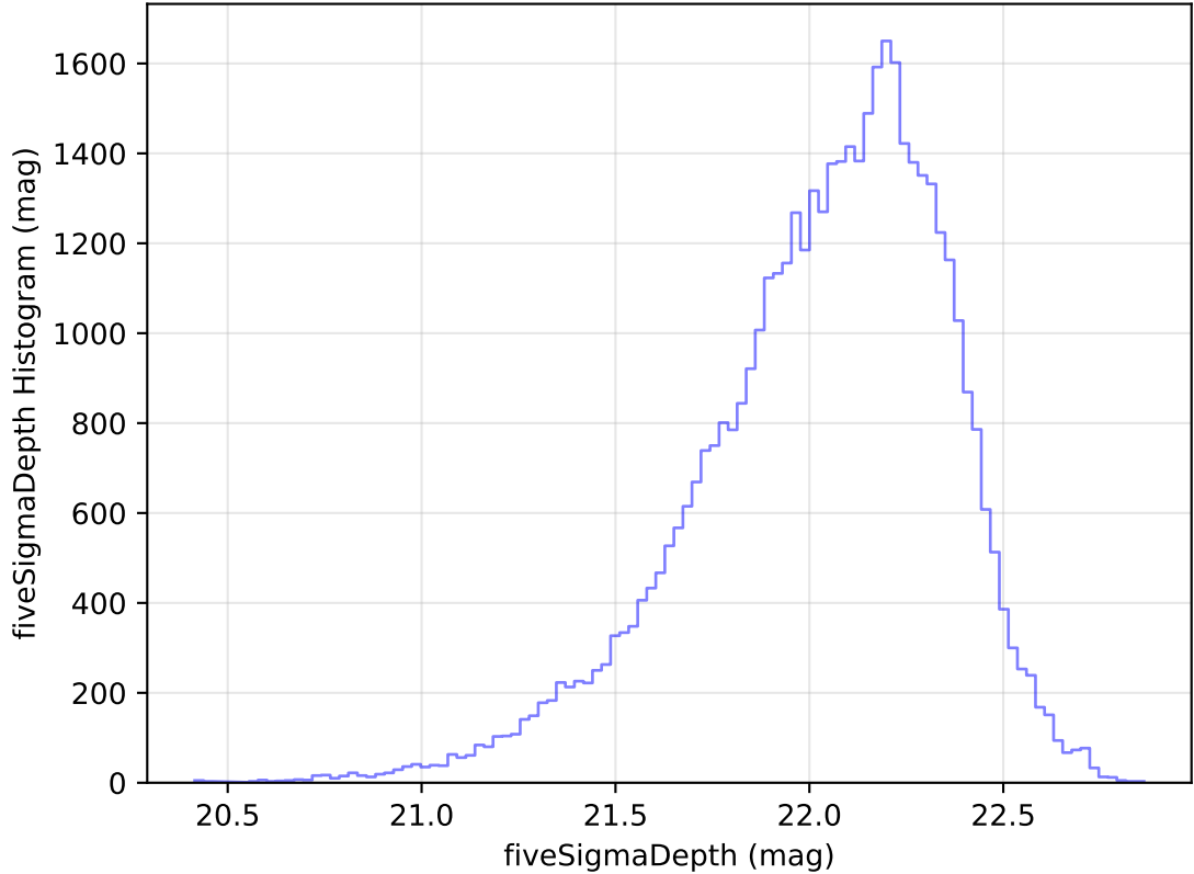
too_elab_heavy_r128_d2_griz_v3.4_10yrs Yr 1 y band: fiveSigmaDepth Histogram
