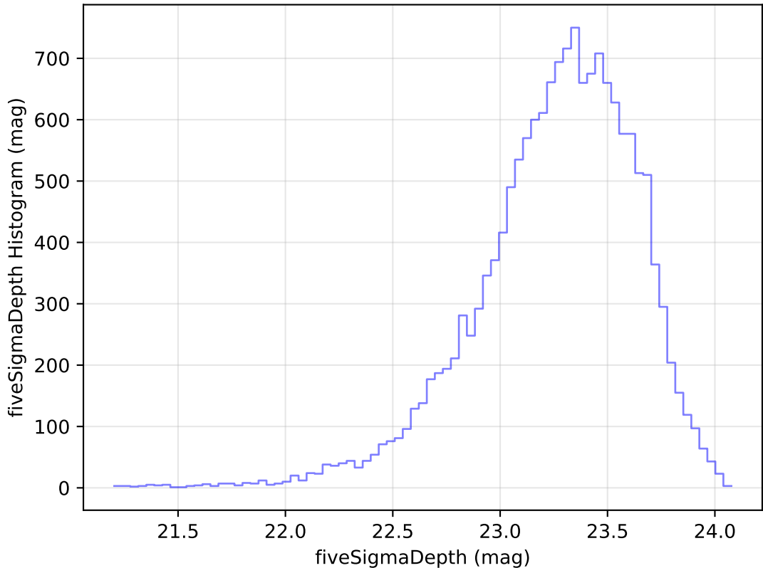
too_elab_heavy_r128_d2_griz_v3.4_10yrs Yr 1 u band: fiveSigmaDepth Histogram
