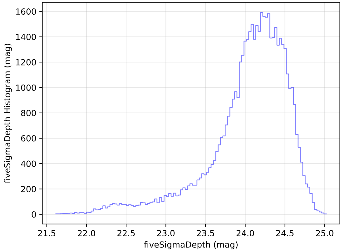
too_elab_heavy_r128_d2_griz_v3.4_10yrs Yr 1 r band: fiveSigmaDepth Histogram
