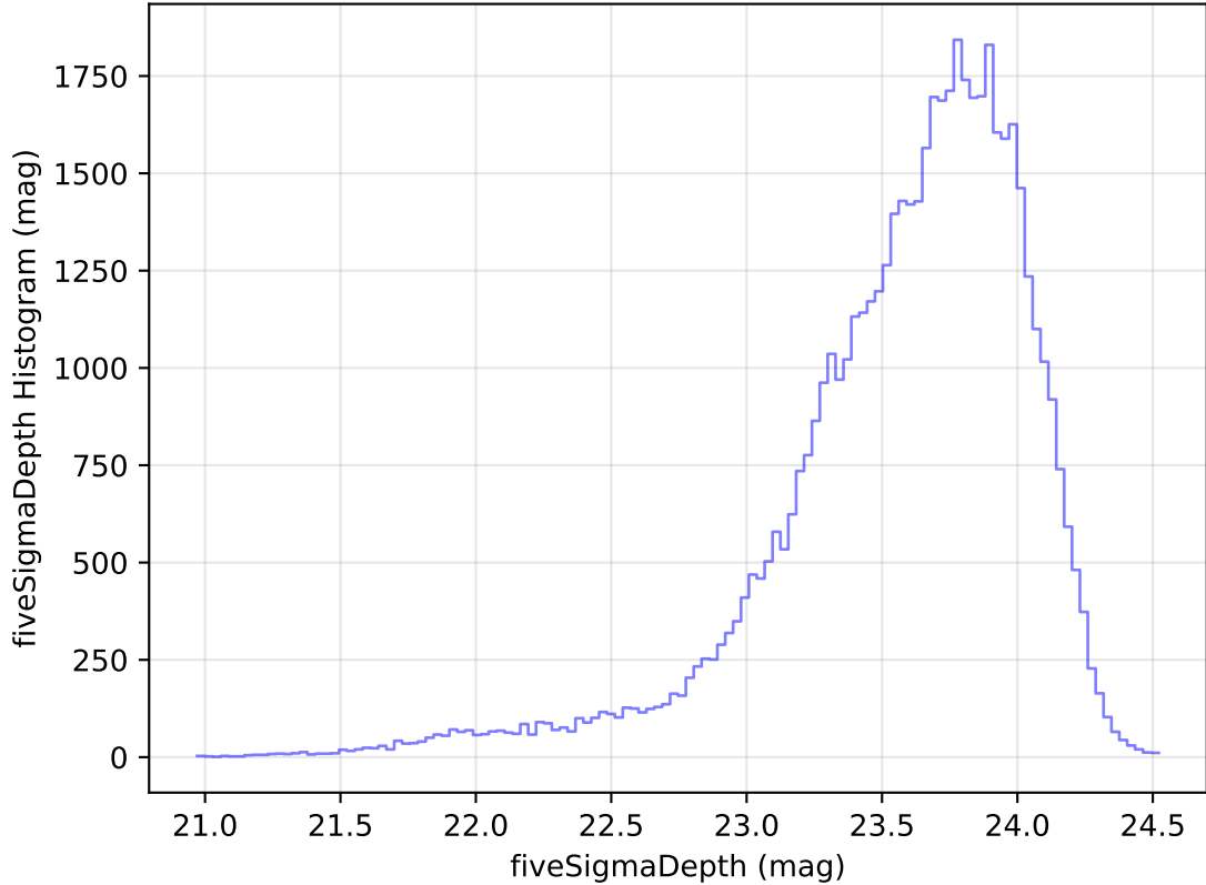
too_elab_heavy_r128_d2_griz_v3.4_10yrs Yr 1 i band: fiveSigmaDepth Histogram
