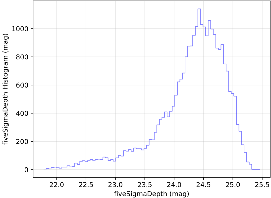
too_elab_heavy_r128_d2_griz_v3.4_10yrs Yr 1 g band: fiveSigmaDepth Histogram
