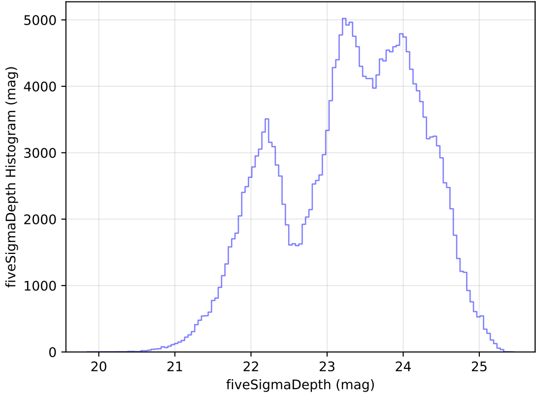
too_elab_heavy_r128_d2_griz_v3.4_10yrs Yr 1 all bands: fiveSigmaDepth Histogram
