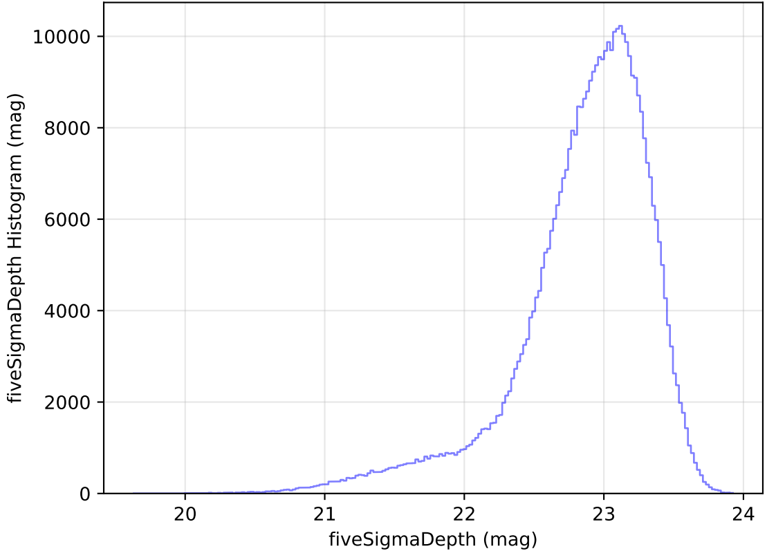
too_elab_heavy_r128_d2_griz_v3.4_10yrs WFD z band: fiveSigmaDepth Histogram
