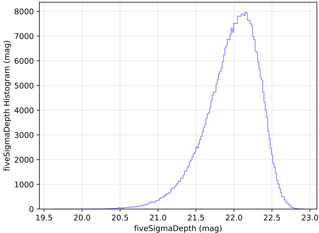
too_elab_heavy_r128_d2_griz_v3.4_10yrs WFD y band: fiveSigmaDepth Histogram
