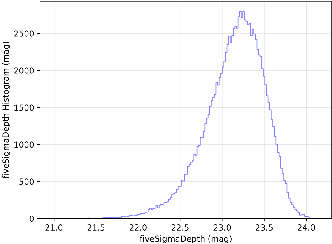
too_elab_heavy_r128_d2_griz_v3.4_10yrs WFD u band: fiveSigmaDepth Histogram
