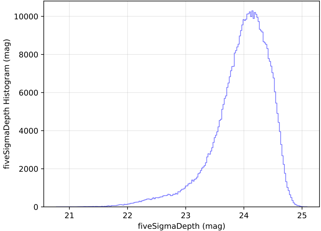
too_elab_heavy_r128_d2_griz_v3.4_10yrs WFD r band: fiveSigmaDepth Histogram
