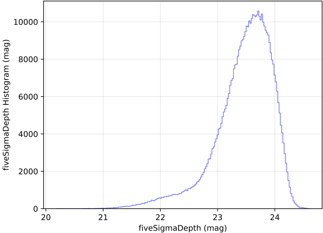
too_elab_heavy_r128_d2_griz_v3.4_10yrs WFD i band: fiveSigmaDepth Histogram
