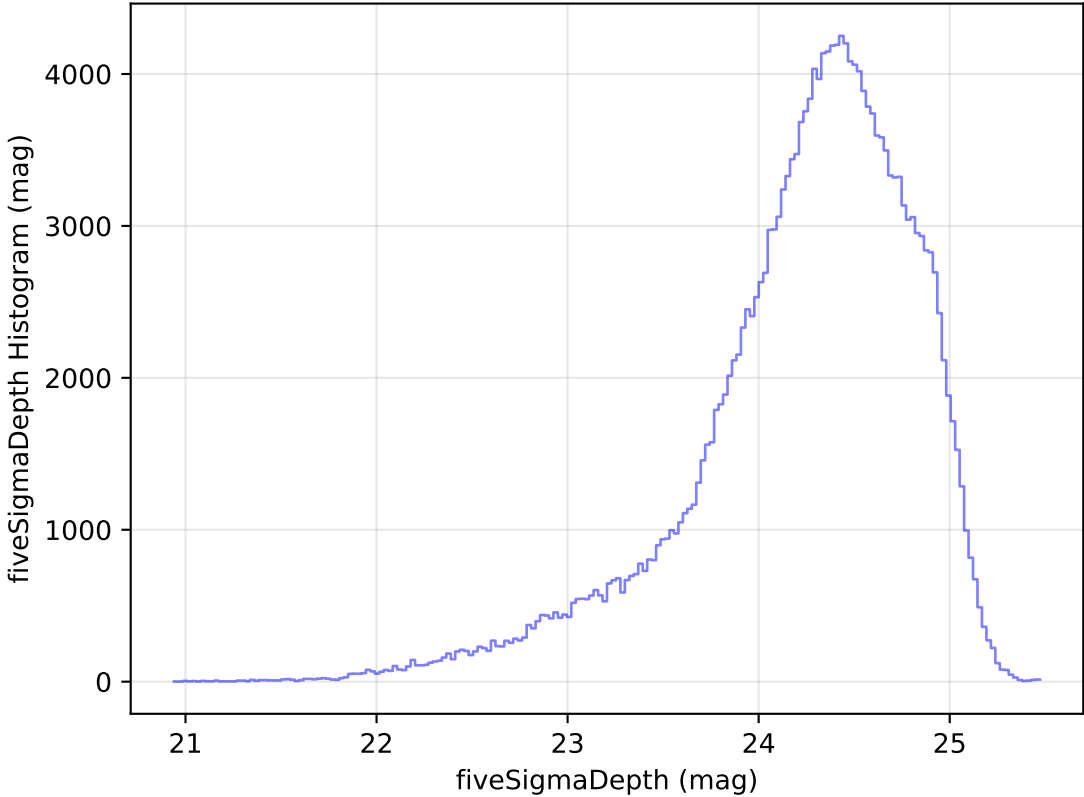
too_elab_heavy_r128_d2_griz_v3.4_10yrs WFD g band: fiveSigmaDepth Histogram
