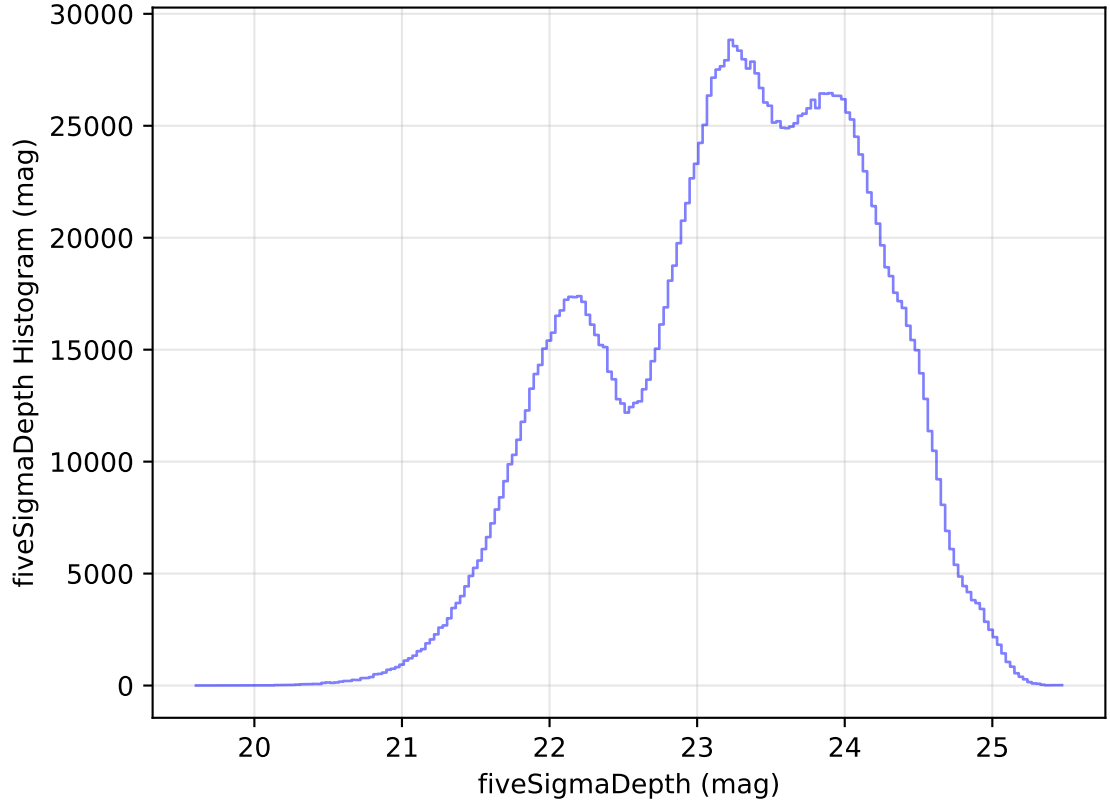
too_elab_heavy_r128_d2_griz_v3.4_10yrs WFD all bands: fiveSigmaDepth Histogram
