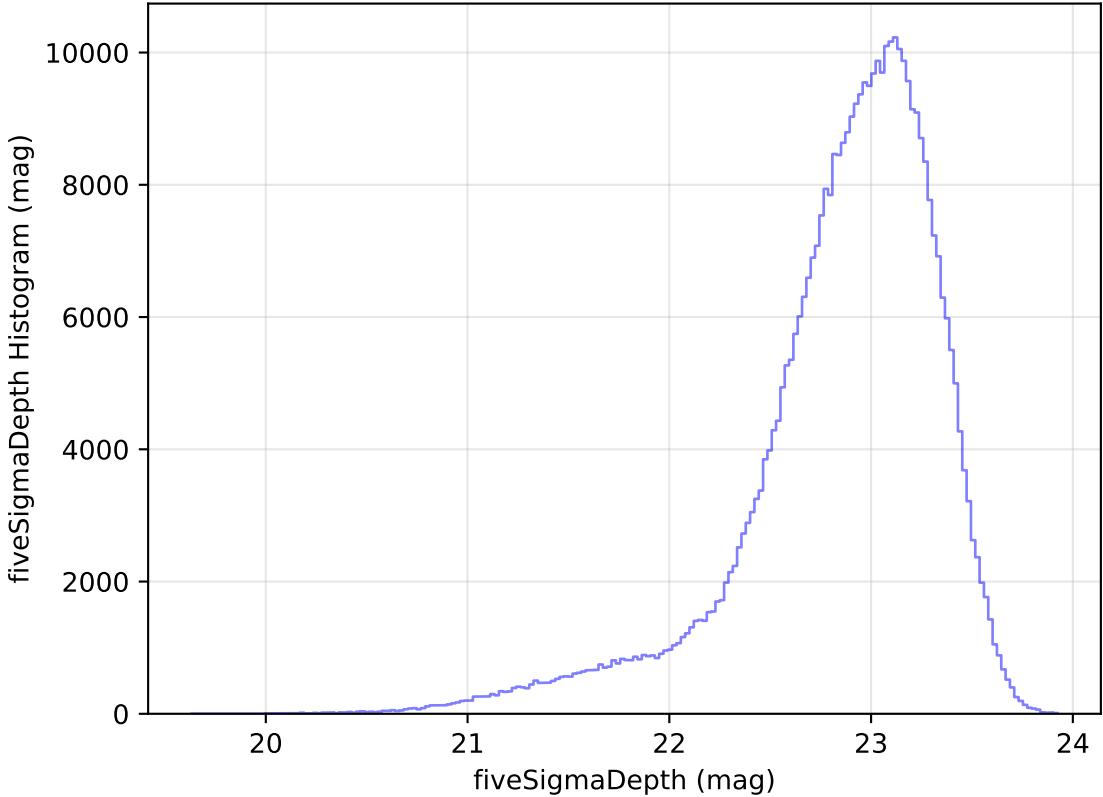
too_elab_heavy_r128_d2_griz_v3.4_10yrs All sky z band: fiveSigmaDepth Histogram
