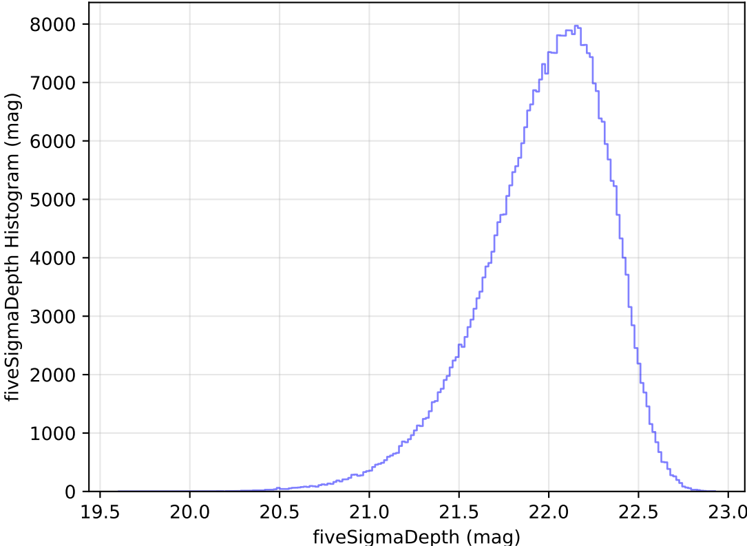
too_elab_heavy_r128_d2_griz_v3.4_10yrs All sky y band: fiveSigmaDepth Histogram
