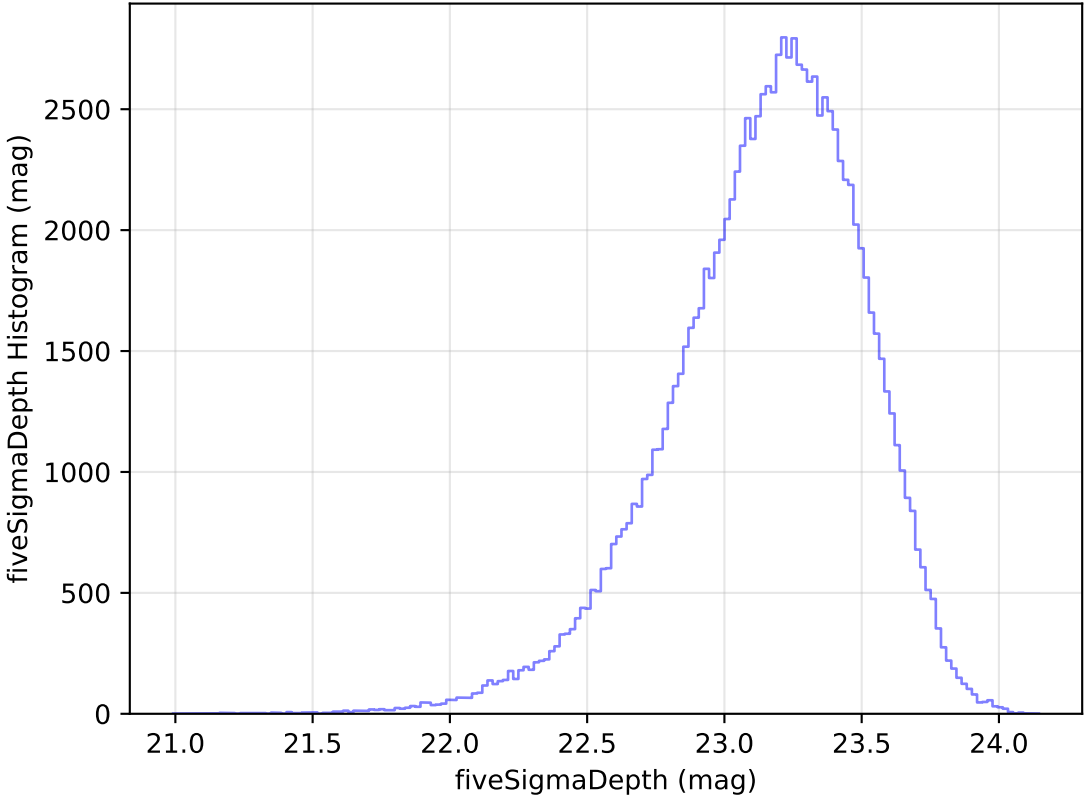
too_elab_heavy_r128_d2_griz_v3.4_10yrs All sky u band: fiveSigmaDepth Histogram
