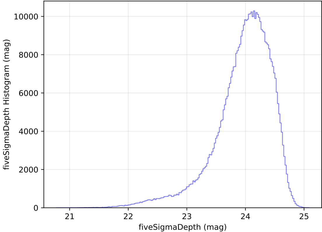
too_elab_heavy_r128_d2_griz_v3.4_10yrs All sky r band: fiveSigmaDepth Histogram
