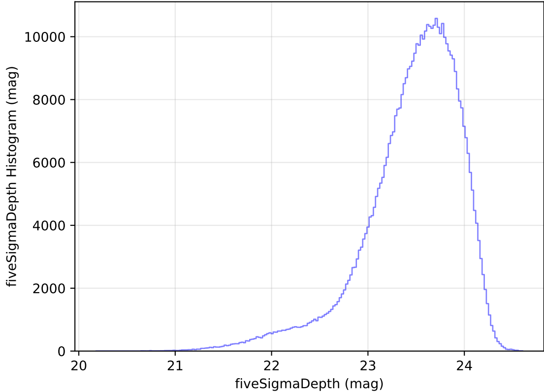
too_elab_heavy_r128_d2_griz_v3.4_10yrs All sky i band: fiveSigmaDepth Histogram
