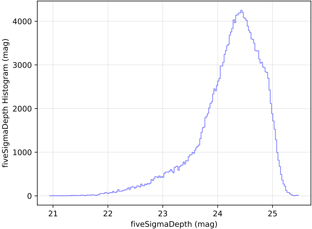
too_elab_heavy_r128_d2_griz_v3.4_10yrs All sky g band: fiveSigmaDepth Histogram
