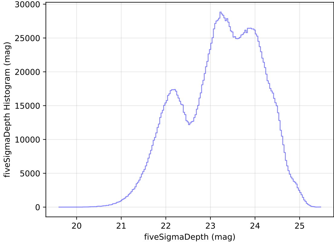
too_elab_heavy_r128_d2_griz_v3.4_10yrs All sky all bands: fiveSigmaDepth Histogram
