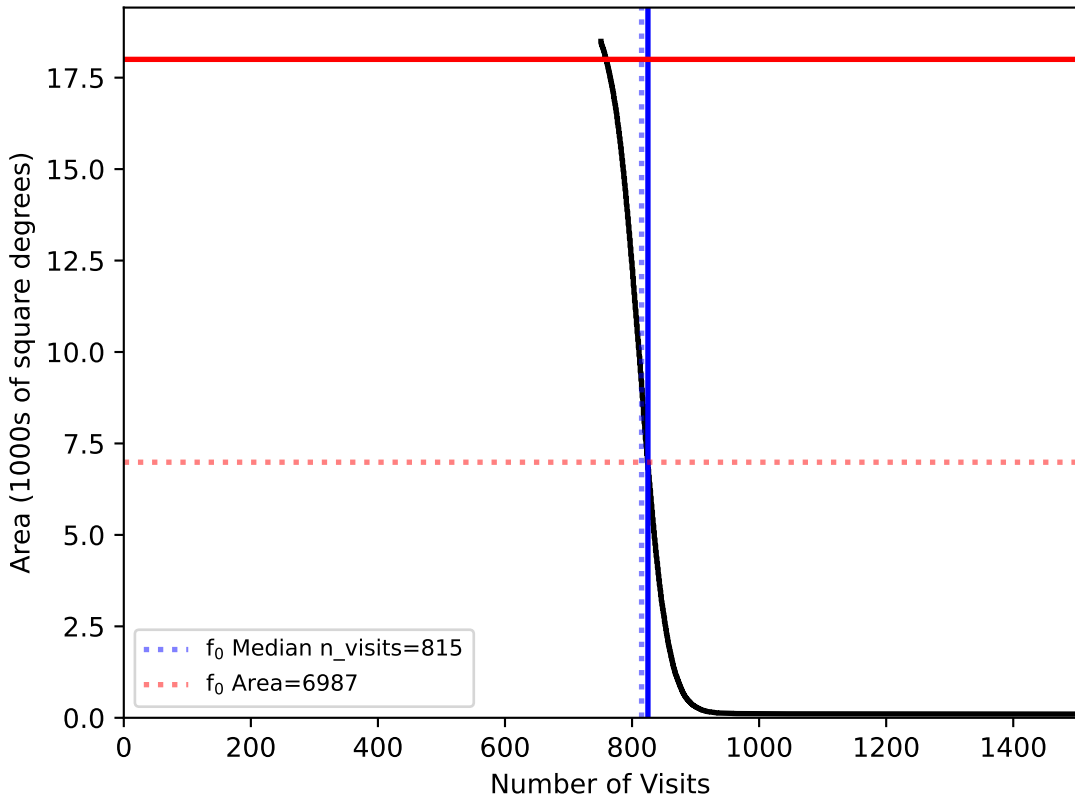
too_elab_heavy_r128_d2_griz_v3.4_10yrs WFD: f0
