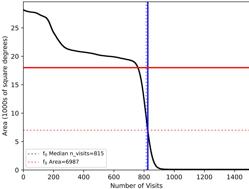
too_elab_heavy_r128_d2_griz_v3.4_10yrs All sky: f0
