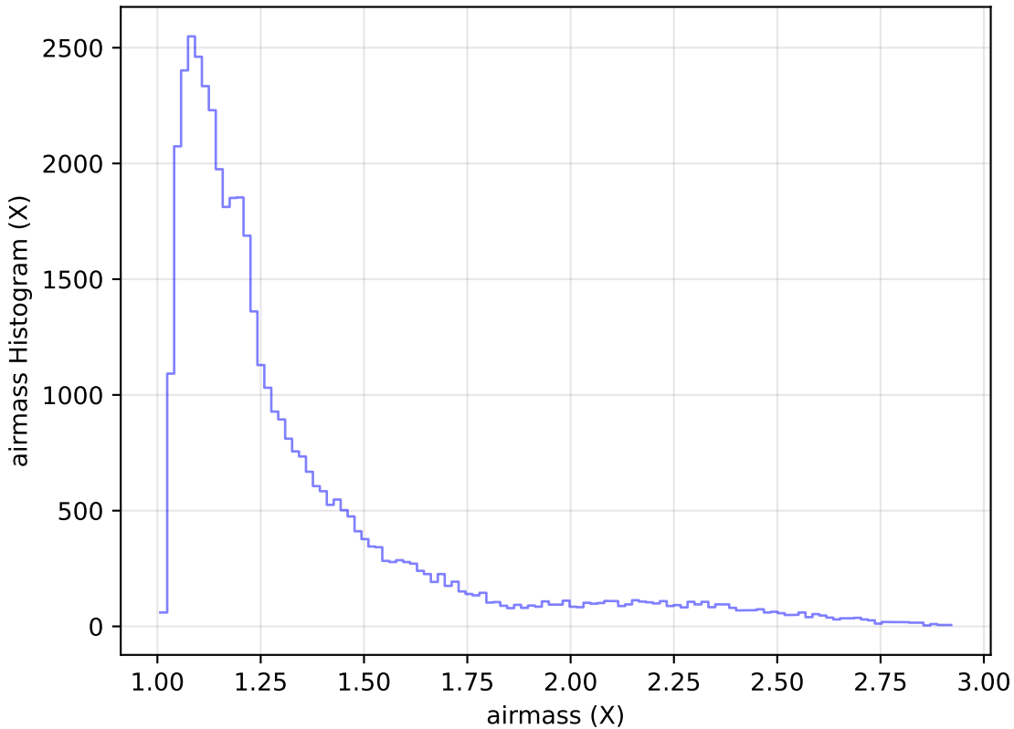
too_elab_heavy_r128_d2_griz_v3.4_10yrs Yr 1 z band: airmass Histogram
