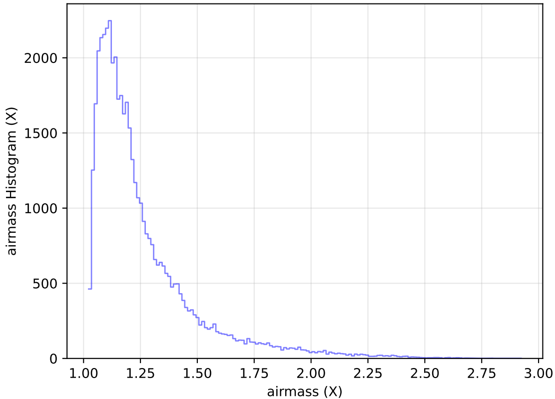
too_elab_heavy_r128_d2_griz_v3.4_10yrs Yr 1 y band: airmass Histogram
