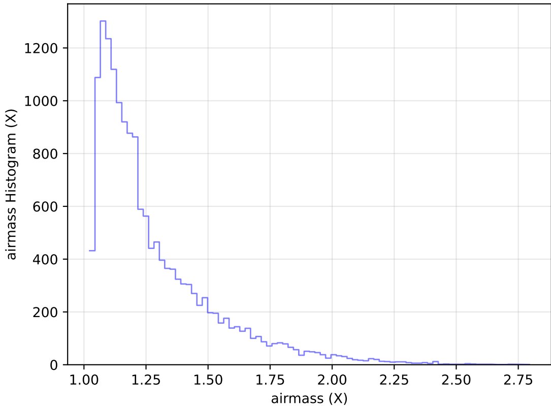
too_elab_heavy_r128_d2_griz_v3.4_10yrs Yr 1 u band: airmass Histogram
