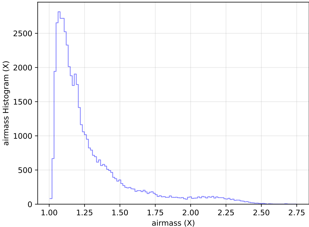
too_elab_heavy_r128_d2_griz_v3.4_10yrs Yr 1 r band: airmass Histogram
