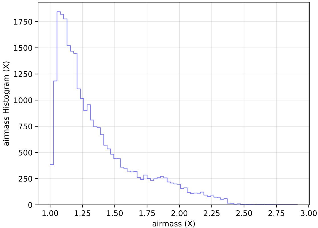
too_elab_heavy_r128_d2_griz_v3.4_10yrs Yr 1 g band: airmass Histogram
