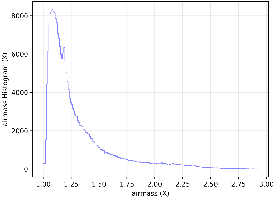
too_elab_heavy_r128_d2_griz_v3.4_10yrs Yr 1 all bands: airmass Histogram
