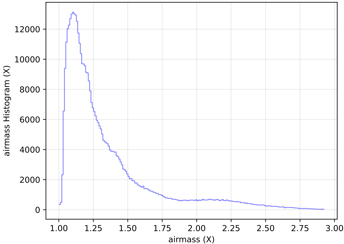
too_elab_heavy_r128_d2_griz_v3.4_10yrs WFD z band: airmass Histogram
