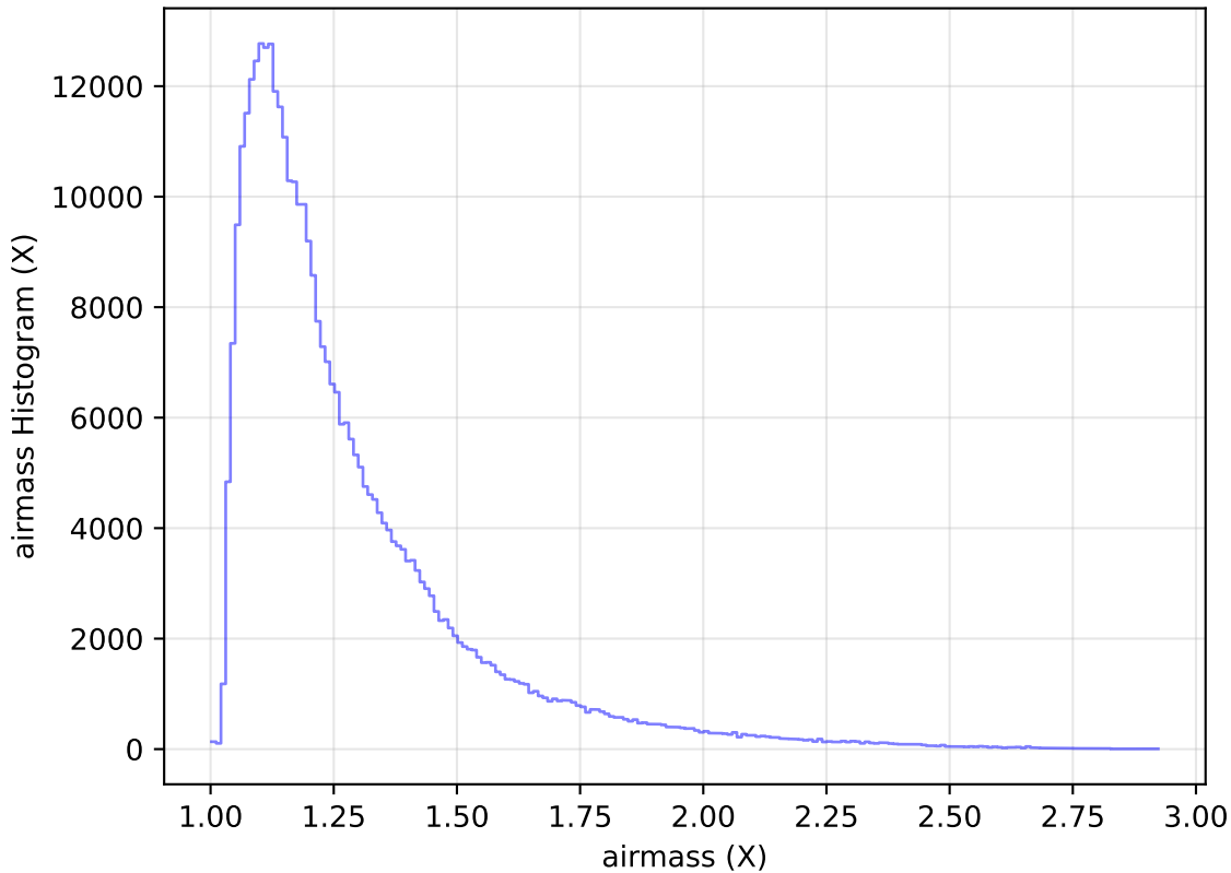
too_elab_heavy_r128_d2_griz_v3.4_10yrs WFD y band: airmass Histogram
