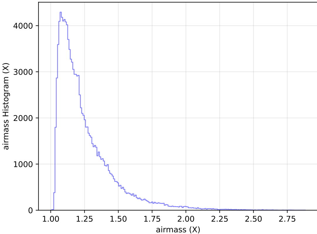
too_elab_heavy_r128_d2_griz_v3.4_10yrs WFD u band: airmass Histogram
