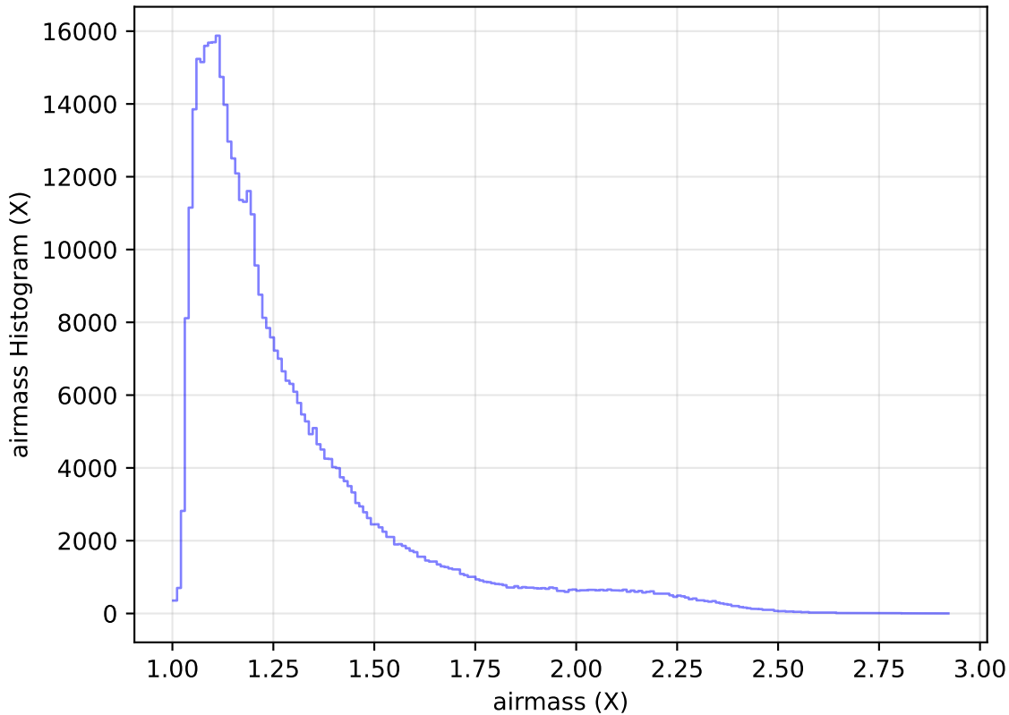
too_elab_heavy_r128_d2_griz_v3.4_10yrs WFD r band: airmass Histogram
