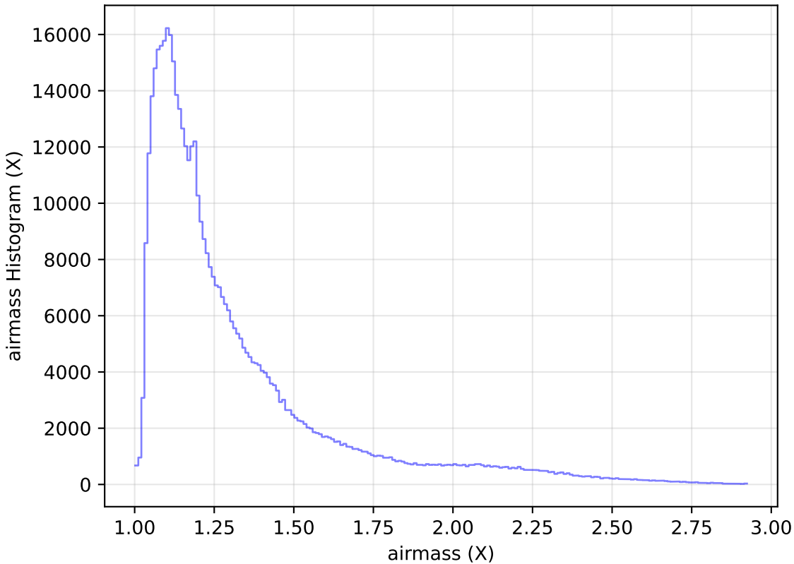
too_elab_heavy_r128_d2_griz_v3.4_10yrs WFD i band: airmass Histogram
