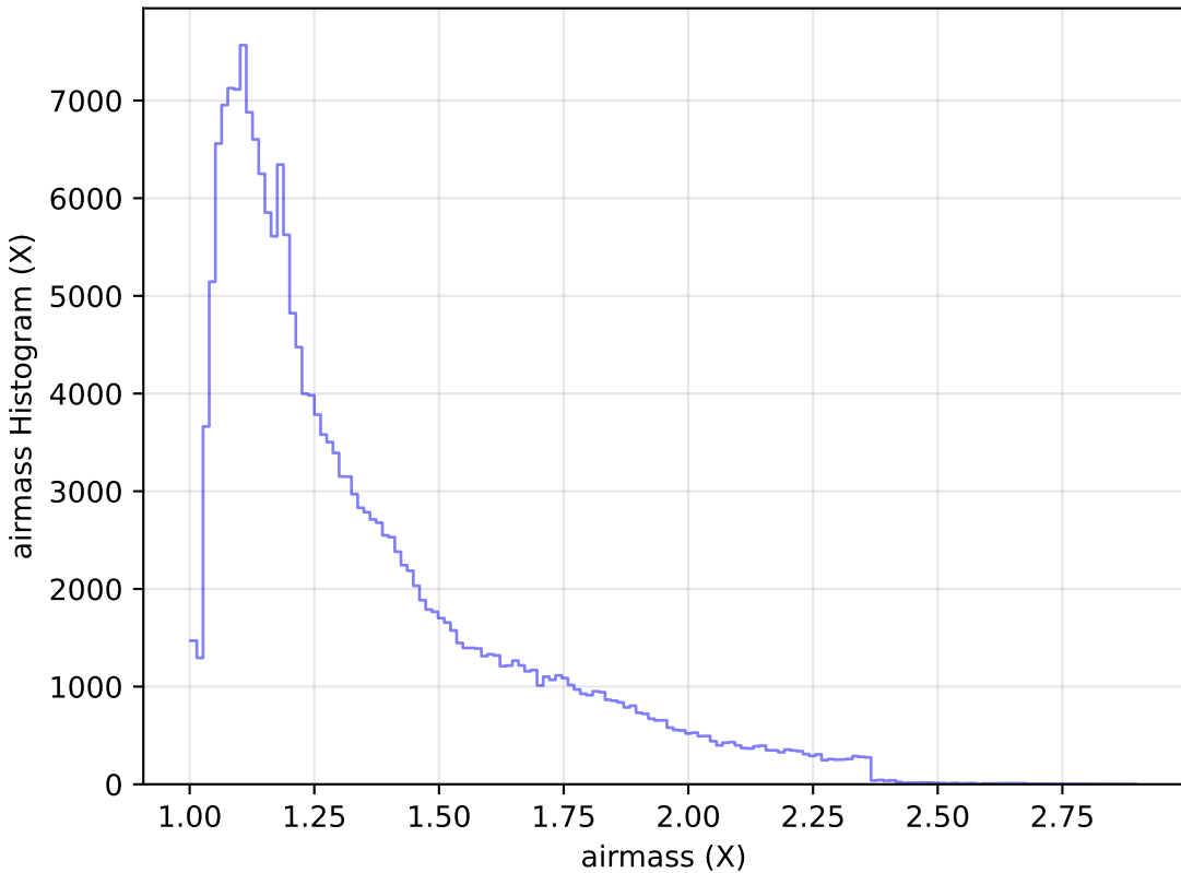
too_elab_heavy_r128_d2_griz_v3.4_10yrs WFD g band: airmass Histogram
