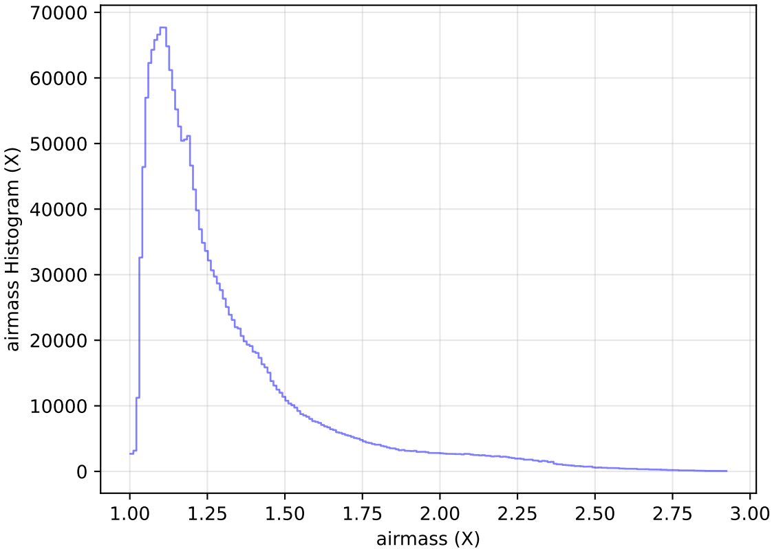
too_elab_heavy_r128_d2_griz_v3.4_10yrs WFD all bands: airmass Histogram
