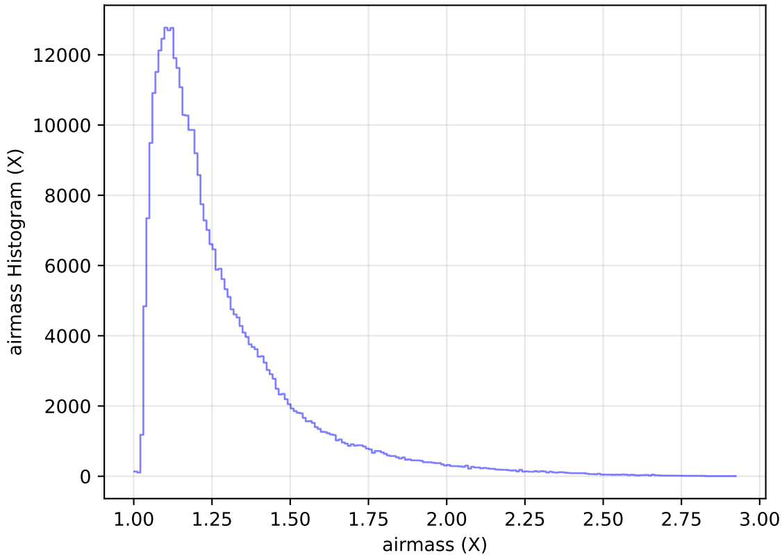
too_elab_heavy_r128_d2_griz_v3.4_10yrs All sky y band: airmass Histogram
