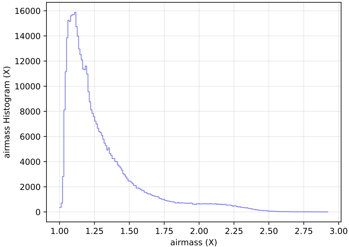
too_elab_heavy_r128_d2_griz_v3.4_10yrs All sky r band: airmass Histogram
